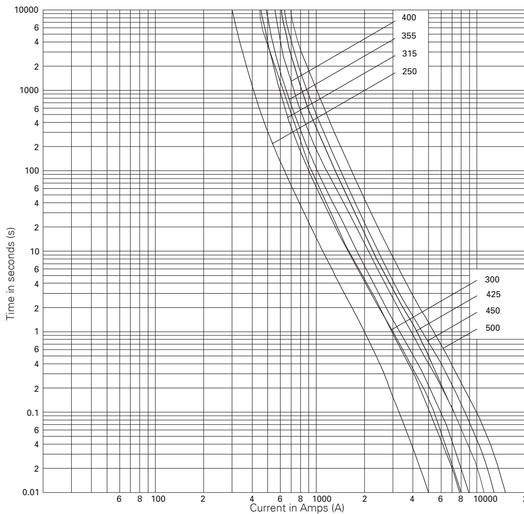
Time-current curves - NH Size 2
