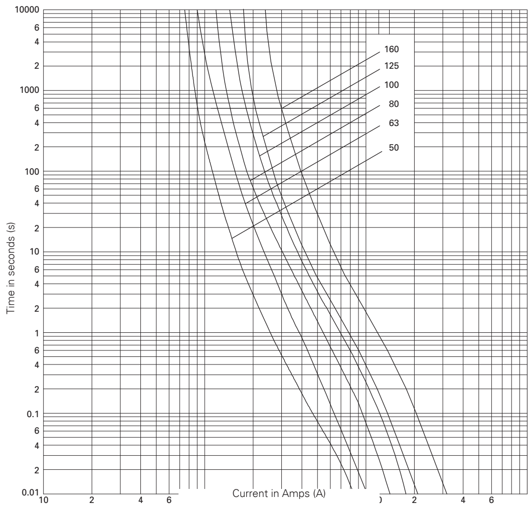
Time-current curves - NH Size 00
