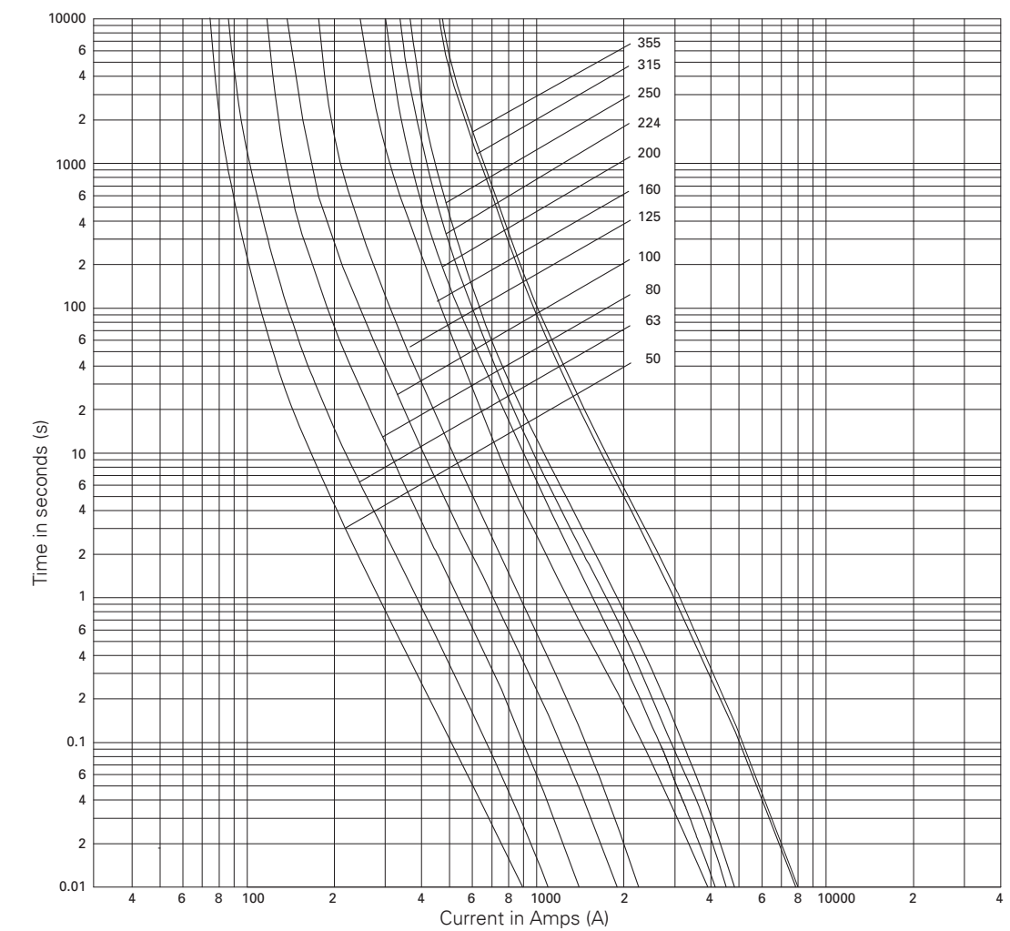
Time-current curves - NH Size 01
